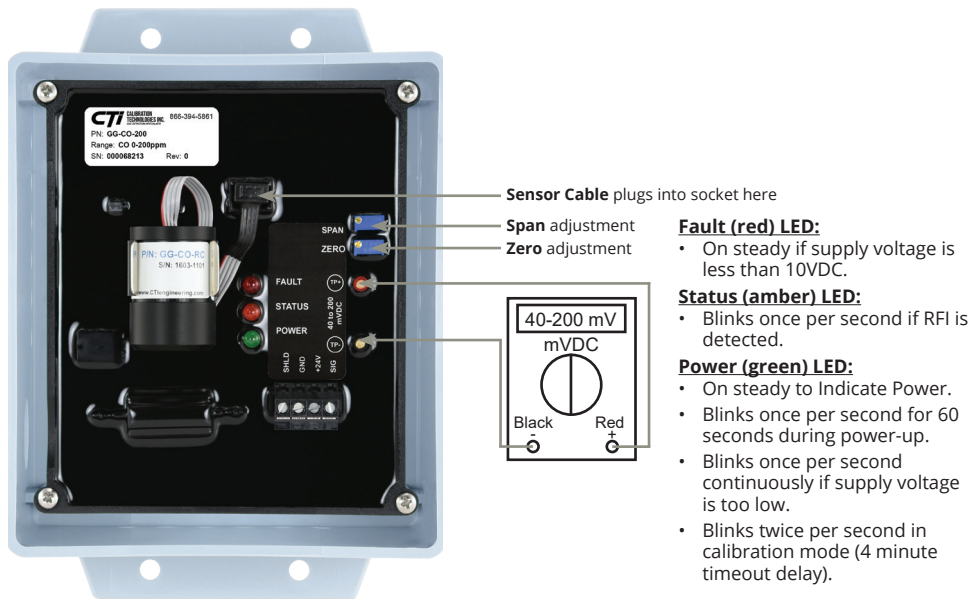
Figure 2: Sensor board components and zero/span adjustment
