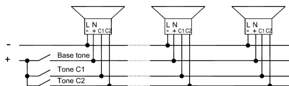
Connection example
